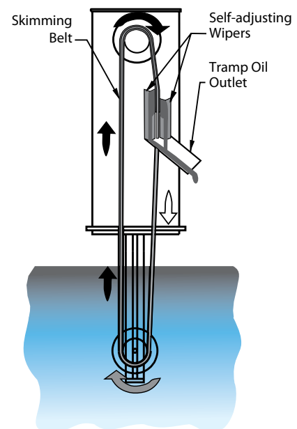
Oil Recovery Unit standard configuration
